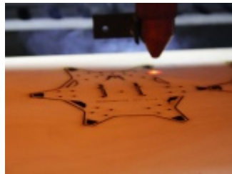
Hexacopter FLT
